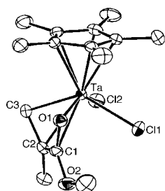
Figure 1. Molecular structure of 2 . Selected bond lengths [Å] and angles [°]: Ta–O1 2.043(3), Ta–C1 2.419(5), Ta–C2 2.403(5), Ta–C3 2.174(5); O1–Ta–C3 76.3(2), C11–Ta–C12 85.39(5), MMA fold angle: 104.2(3).
